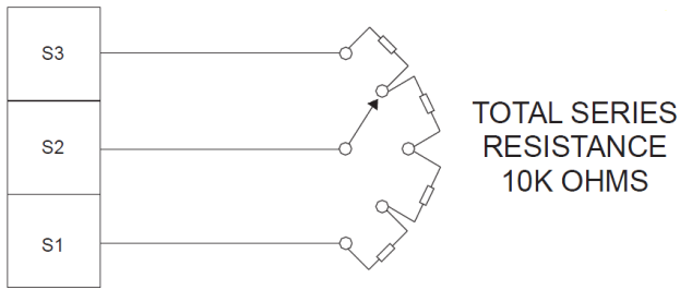
Figure 14. Multiple Fixed Speeds
